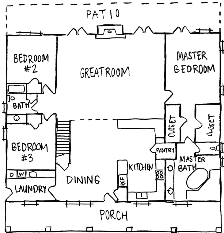
MAIN FLOOR 2668 SF
