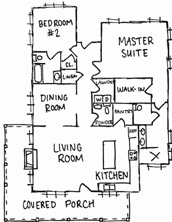
MAIN FLOOR 1688 SF
